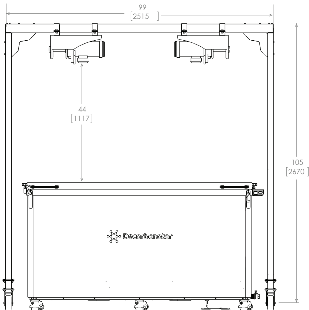
FRONT ELEVATION
