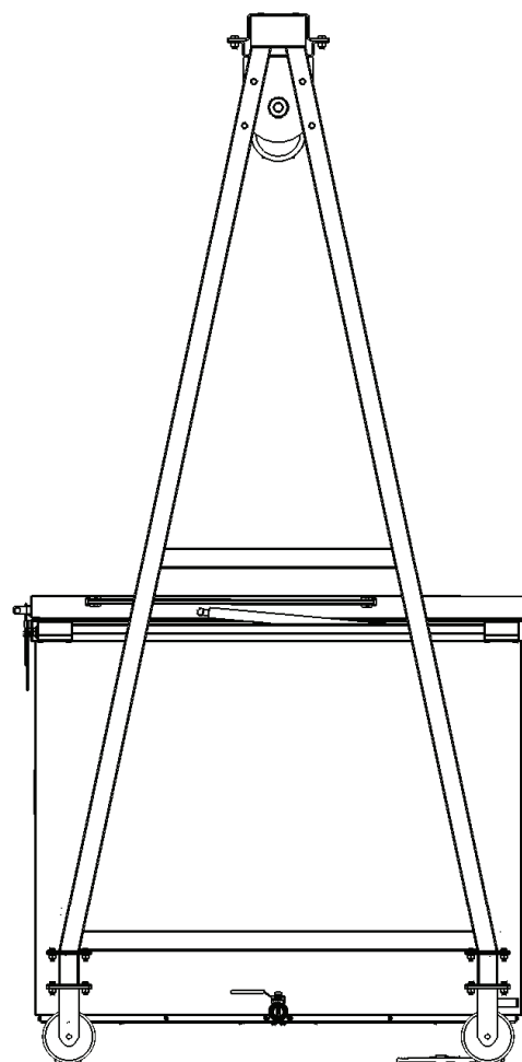
SIDE ELEVATION
